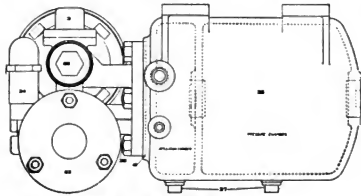
Fig. 2488. Distributing Valve and Double Chamber Reservoir.
